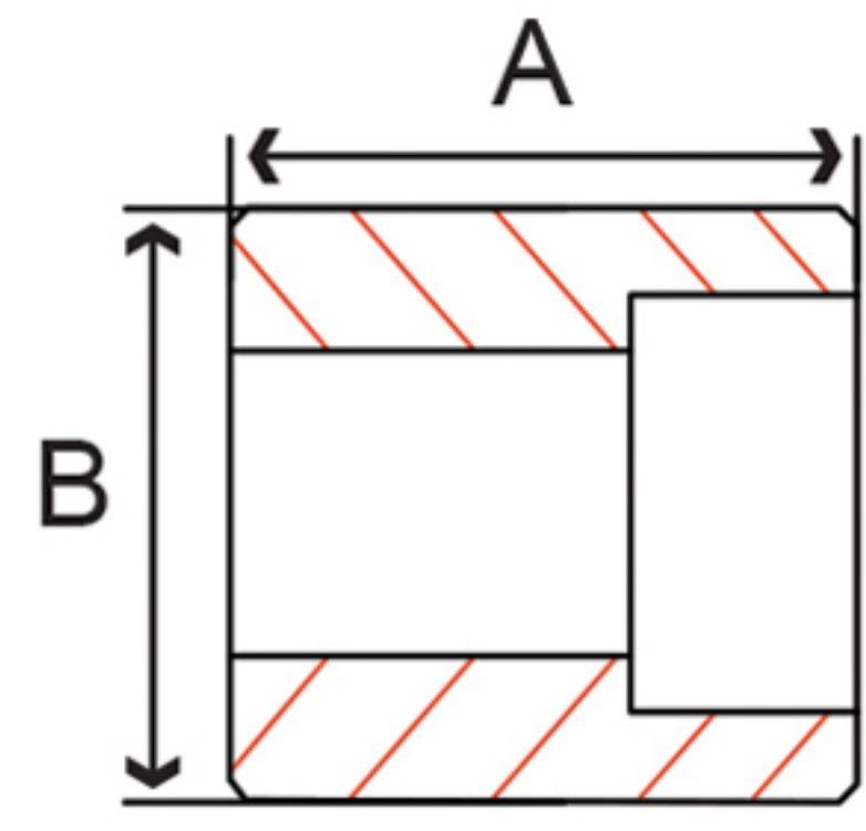
Fig. 52HC3 – Half Coupling
